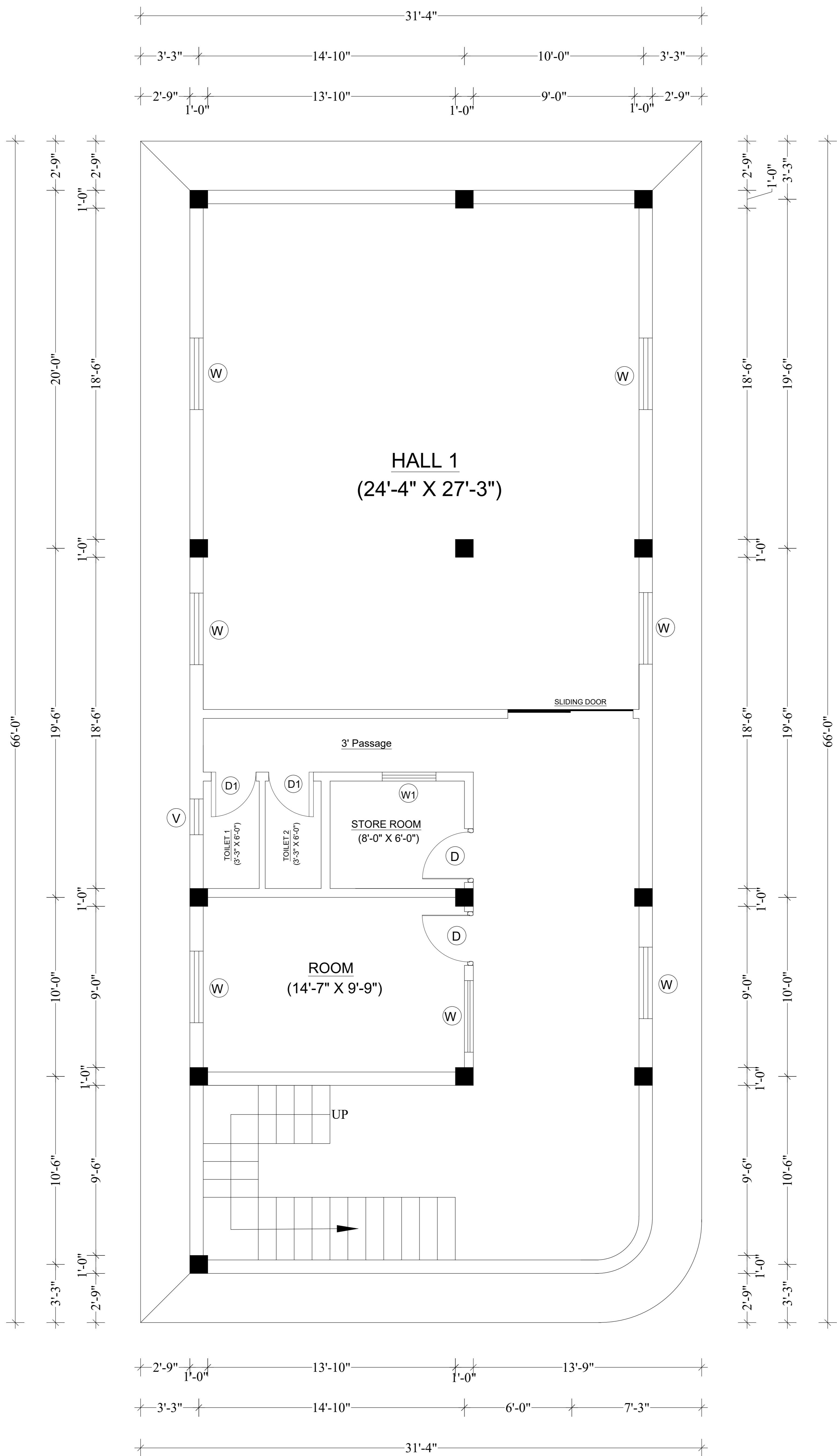
SECOND FLOOR PLAN 2072.26 Sq. ft.
